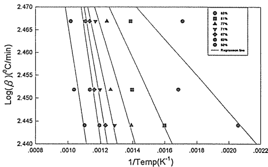
Fig. 5. Plot of slopes used to determine activation energy by Flynn and Wall's method (●) : 95%, (■) : 81%, (▲) : 77%, (▼) : 71%, (◆) : 67%.
