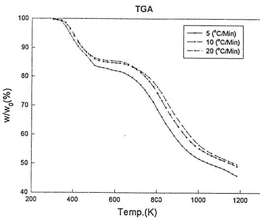
Fig. 2. TGA diagrams for SC-1008 cured phenol resin at several heating rate (●) : 5°C/min, (■) : 10°C/min, (▲) : 20°C/min
