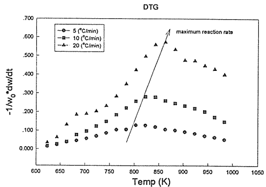
Fig. 4. Rate of weight loss for SC-1008 cured phenol resin (●) : 5°C/min, (■) : 10°C/min, (▲) : 20°C/min.
