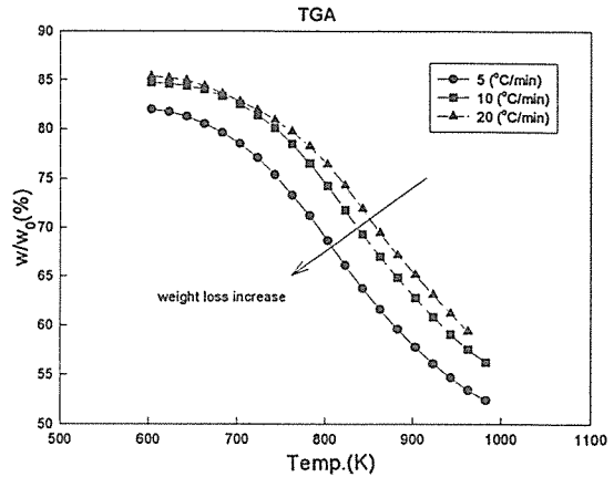
Fig. 3. TGA diagrams in the range of analysis temperature zone (●) : 5°C/min, (■) : 10°C/min, (▲) : 20°C/min.
