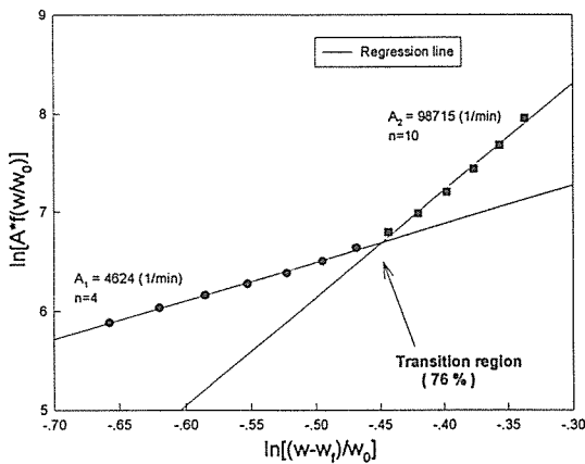
Fig. 7. Plot to determination frequency factor and order of reaction for two region of weight loss (—) : Regression line.
