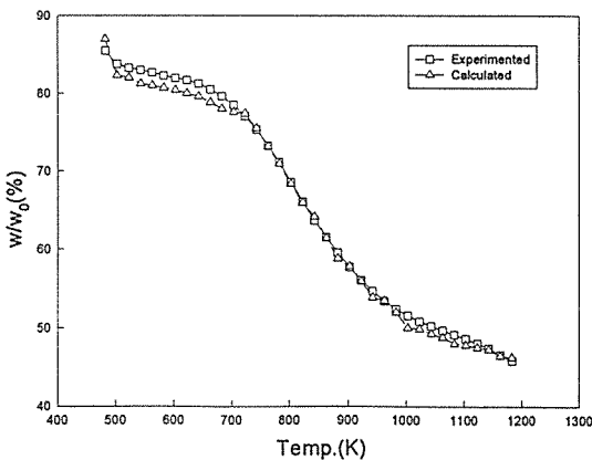
Fig. 8. Comparison of calculated and experimental weight loss curves at 20 °C/min (□) : Experimented, (△) : Calculated.
