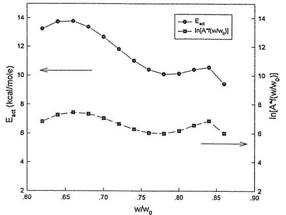
Fig. 6. Activation energy and intercept as a function of degree of conversion (●) : E act , (■) : ln[A*f(w/w 0 )].
