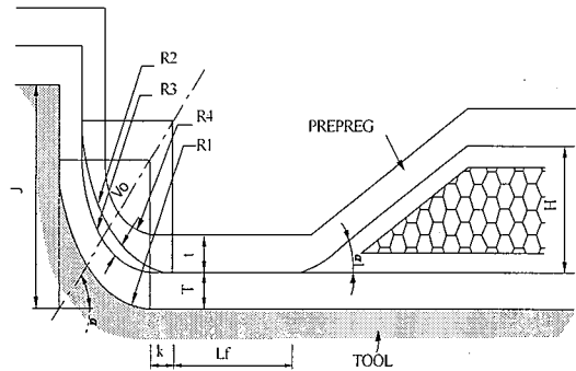
Fig. 5 Schematic diagram of defect at sandwich structure.
