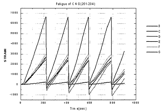
Fig. 12 Typical burst test result and strain readings during fatigue test.
