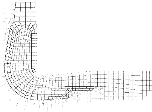
Fig. 4 Modeling with one half of the boss.
