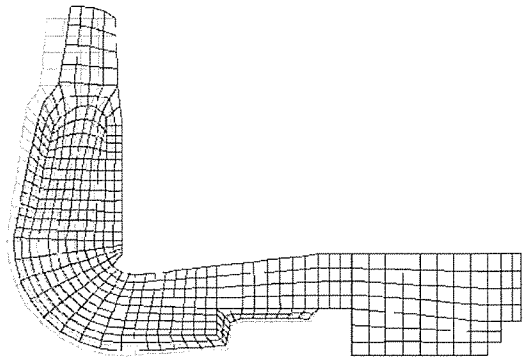
Fig. 5 Deformations after FEM analysis.
