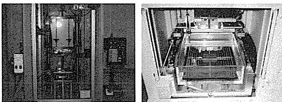
Fig. 3 Impact test machine and damage detection system.
