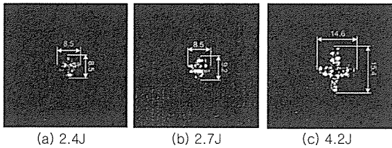
Fig. 12 Delamination area after low velocity impact for [fill2/warp2]s.
