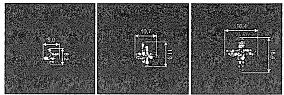
Fig. 10 Delamination area after low velocity impact for [fill]_8 .
