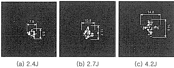
Fig. 13 Delamination area after low velocity impact for [fill/warp/fill/warp]s.
