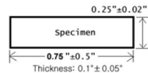
Fig. 2 The measurement of ILSS specimen
