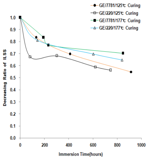
Fig. 8 ILSS behaviors in glass/epoxy specimens.
