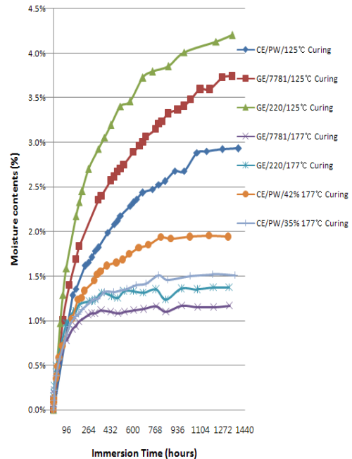
Fig. 3 Water absorption behaviors of the specimens
