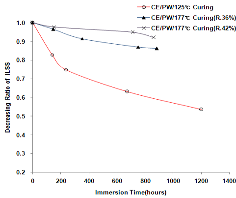
Fig. 7 ILSS behaviors in carbon/epoxy specimens.
