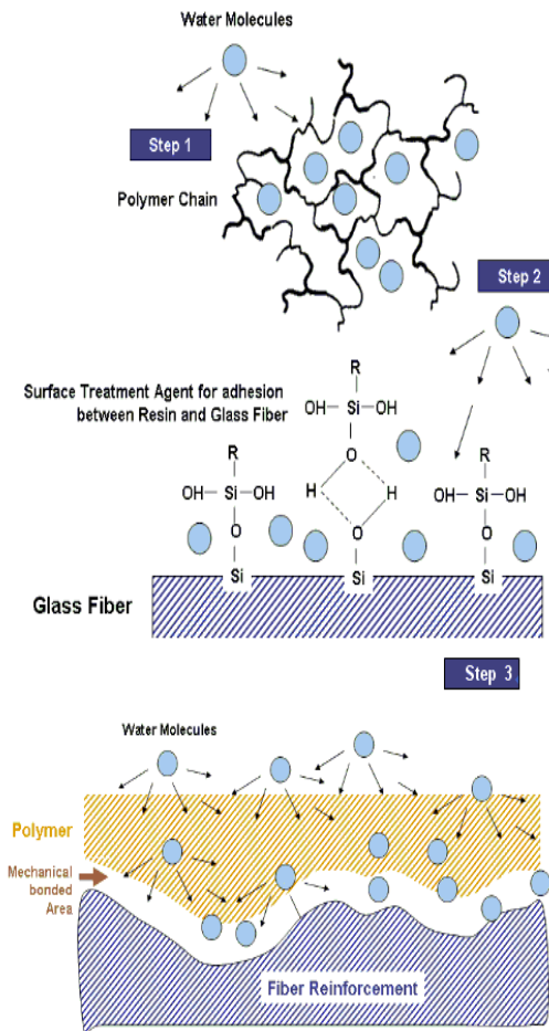
Fig. 6 The process of moisture absorption in the FRP.
