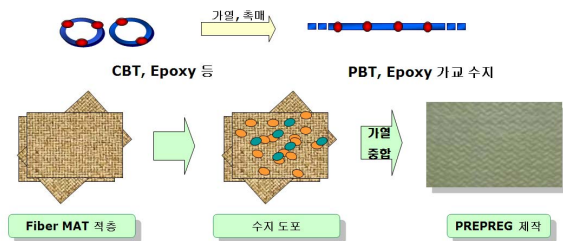
Fig. 1 Manufacturing process of fiber reinforced composite materials.
