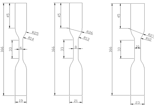
Fig. 3 Three types of tensile specimens used for high strain rate tests.
