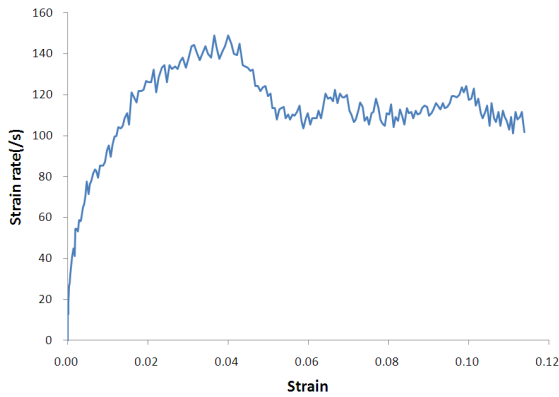
Fig. 7 Variation of strain rate w.r.t strain.
