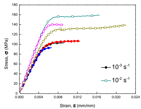
Fig. 7 Stress-strain curves for tibia by strain rates.
